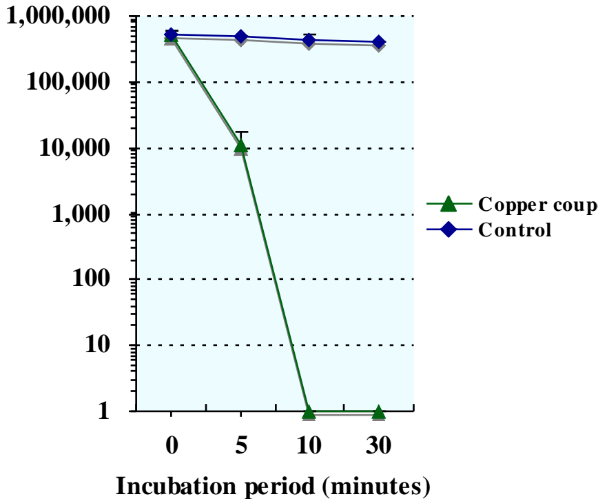
FIGURE 7: MRSA Viability on Copper Alloys and Stainless Steel at 68°F (20°C)**
